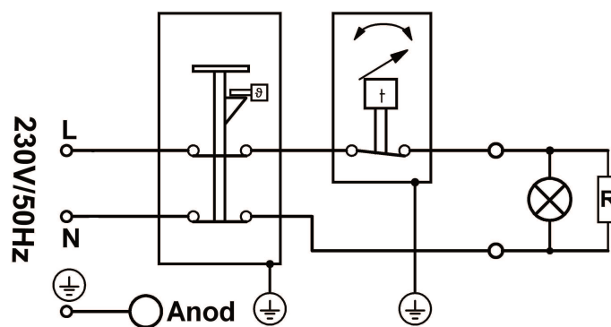
Connection diagram
